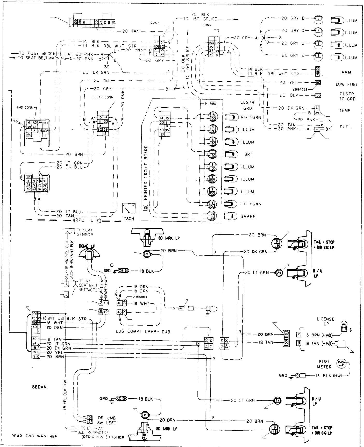
Fig. 105—Body & Rear Lighting (Nova)
