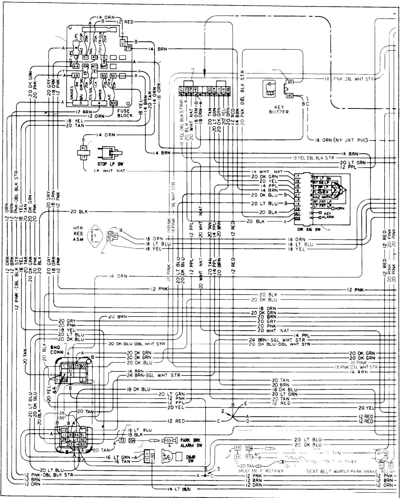
Fig. 103—Instrument Panel (Nova)
