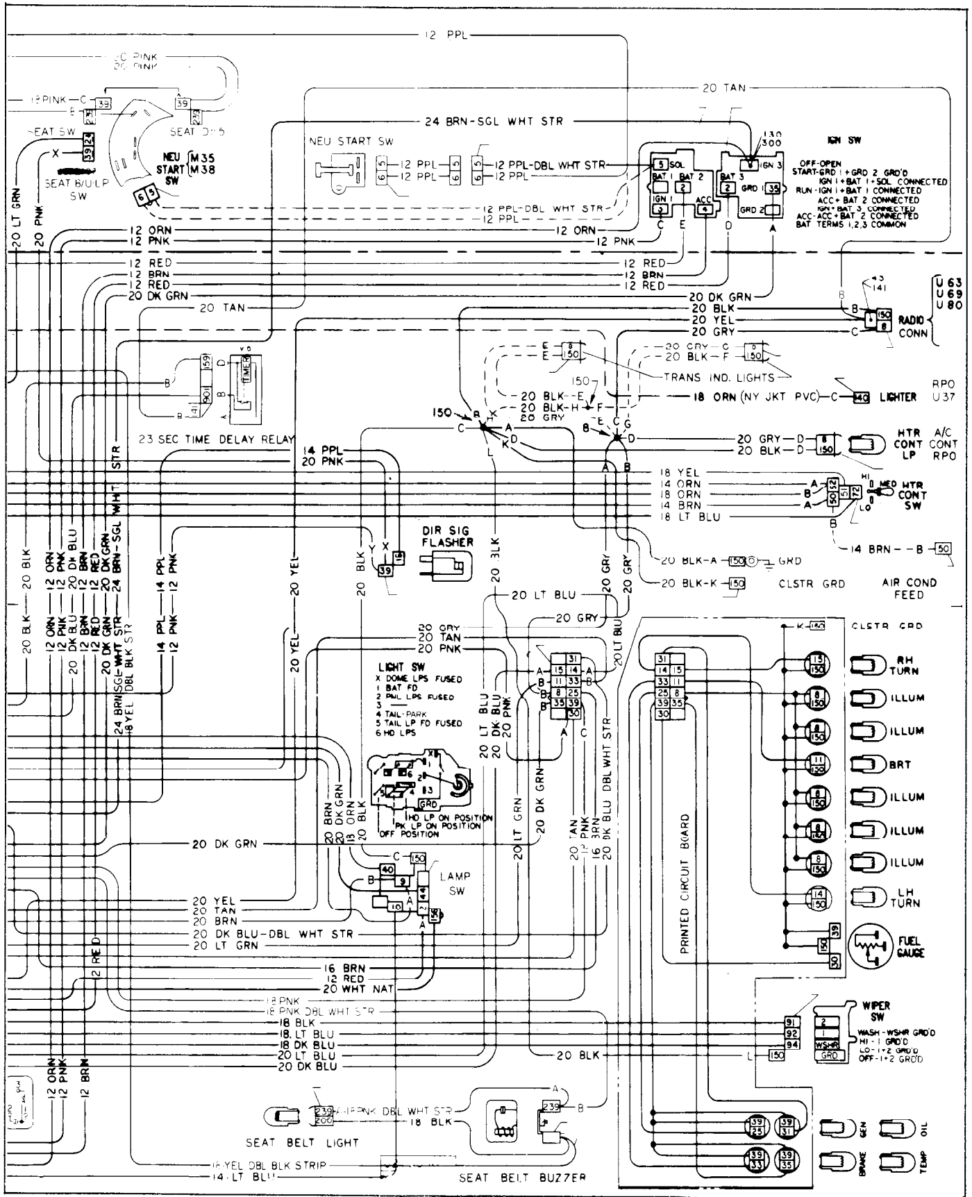
Fig. 104—Instrument Cluster (Nova)
