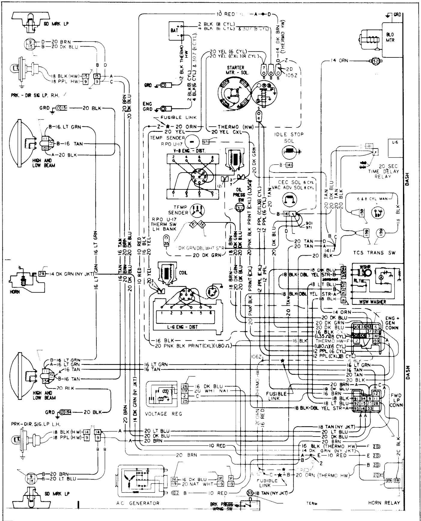
Fig. 102—Engine Compartment (Nova)
