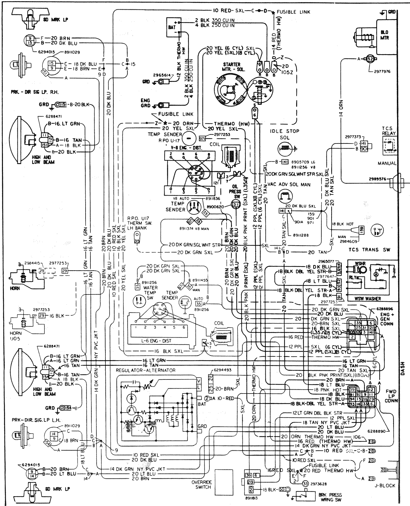
Engine Compartment—Nova
