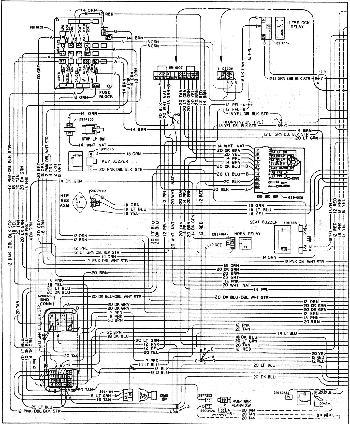
Instrument Panel—Nova
