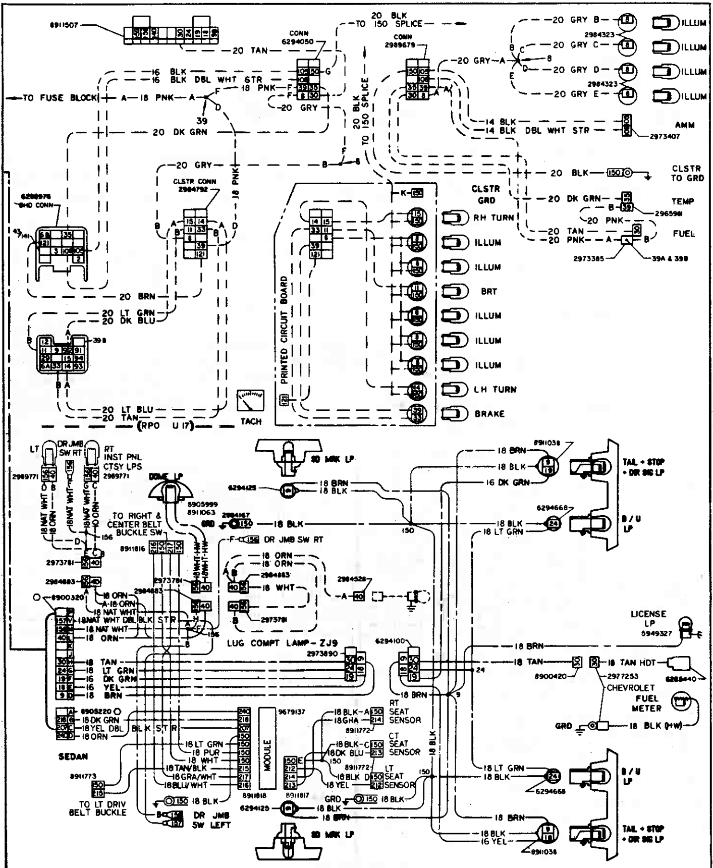
Body & Rear Lighting—Nova
